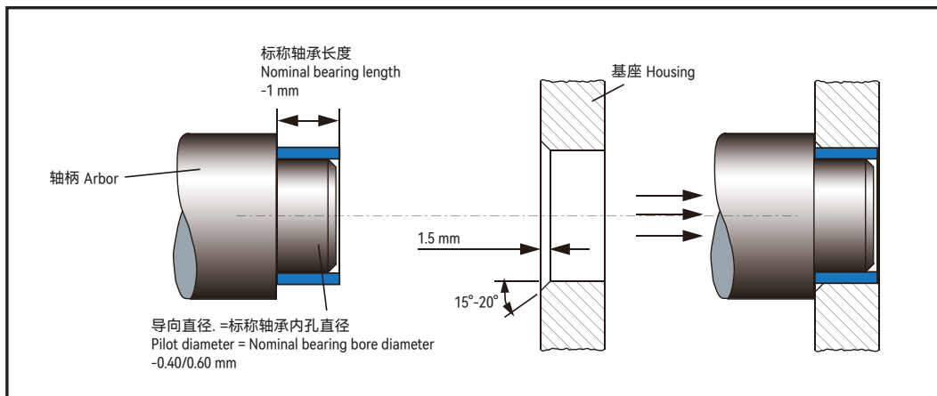
轴承的安装 Bearing Installation
