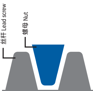
TLS特殊圆角齿形 TLS special tooth with rounded corners
