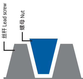
标准梯形齿形 Standard trapezoidal tooth
