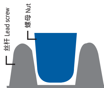
HLS高螺旋线圆齿 TLS high-helix and rounded tooth
